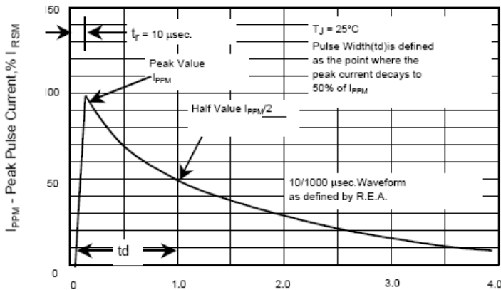
Fig.3 - Pulse Waveform
