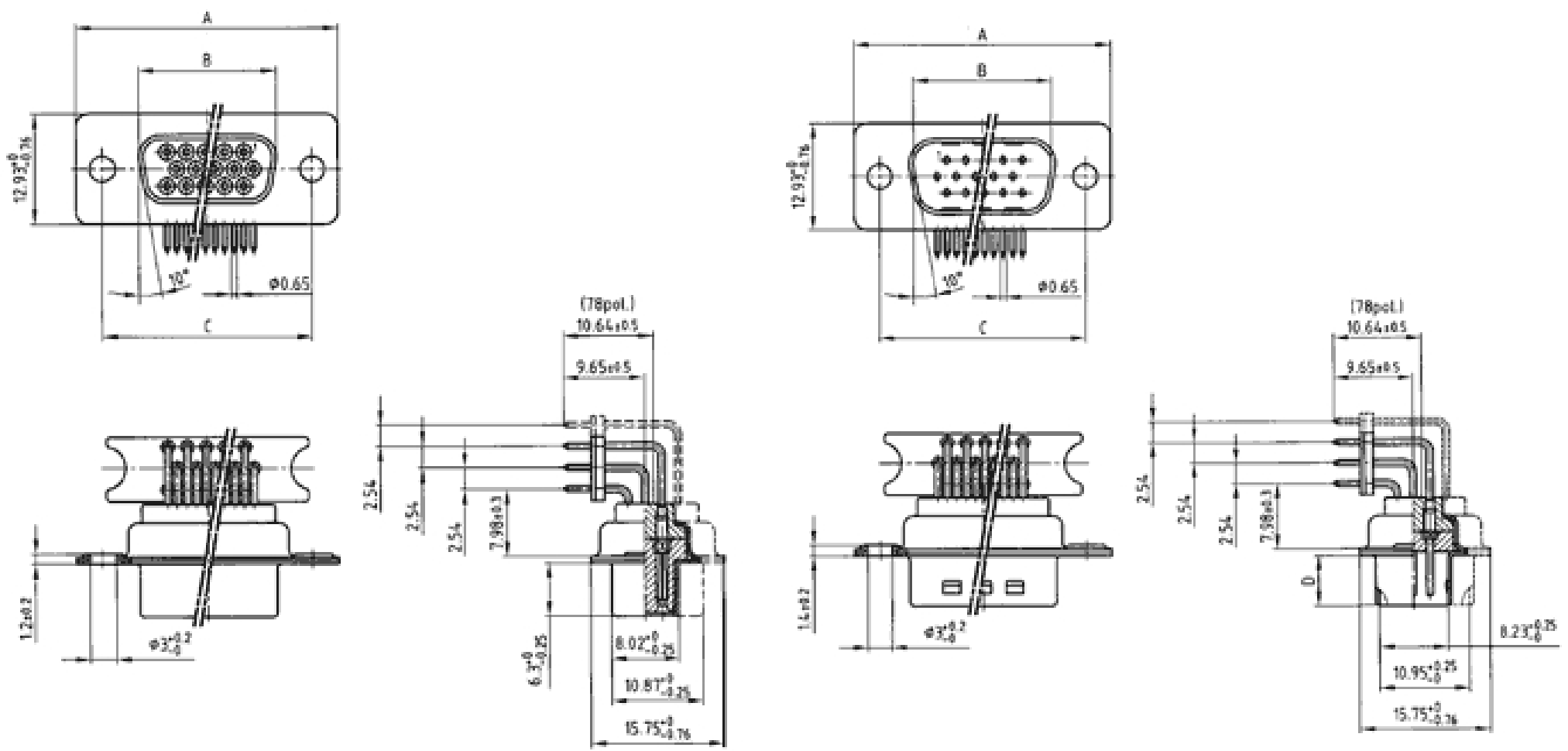
Socket connector:
