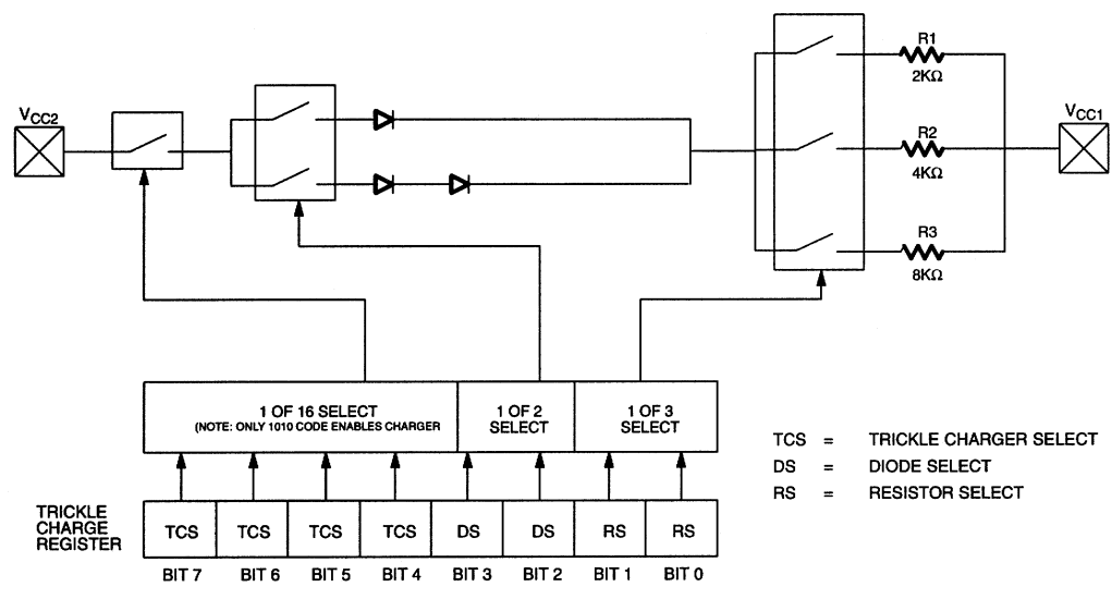
DS1302 PROGRAMMABLE TRICKLE CHARGER Figure 5
