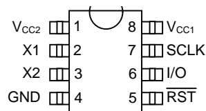
DS1302Z 8-Pin SOIC (150 mil)
