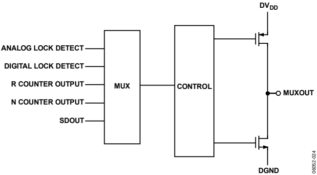
Figure 15. MUXOUT Circuit
