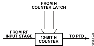
Figure 13. N Counter
