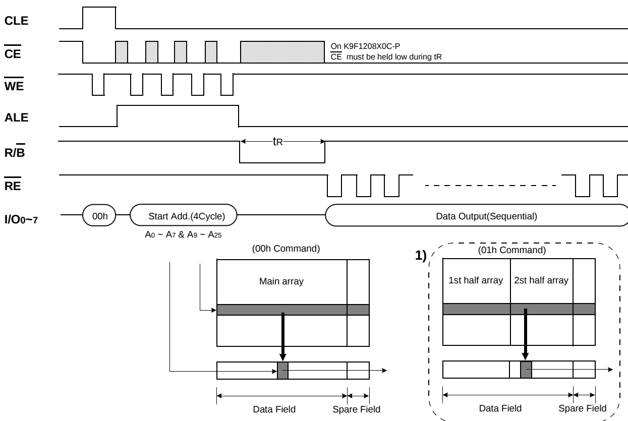
Figure 7. Read1 Operation
