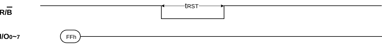
Figure 7. RESET Operation
