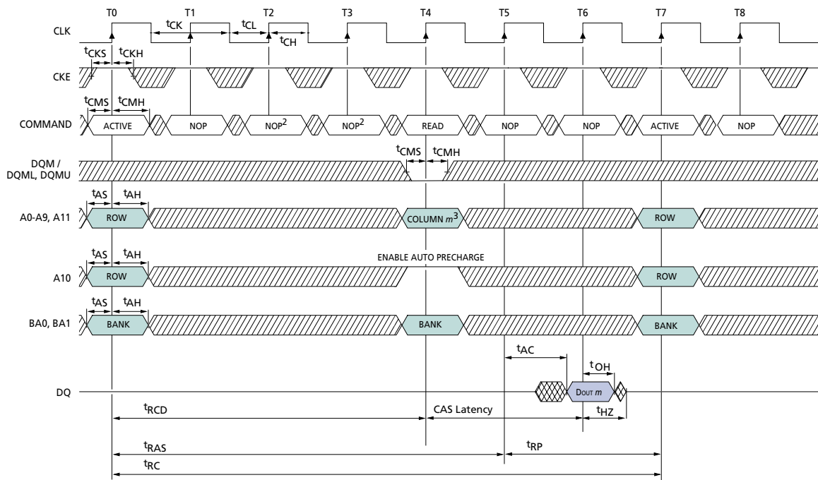
Figure 42: Single Read – With Auto Precharge 1
