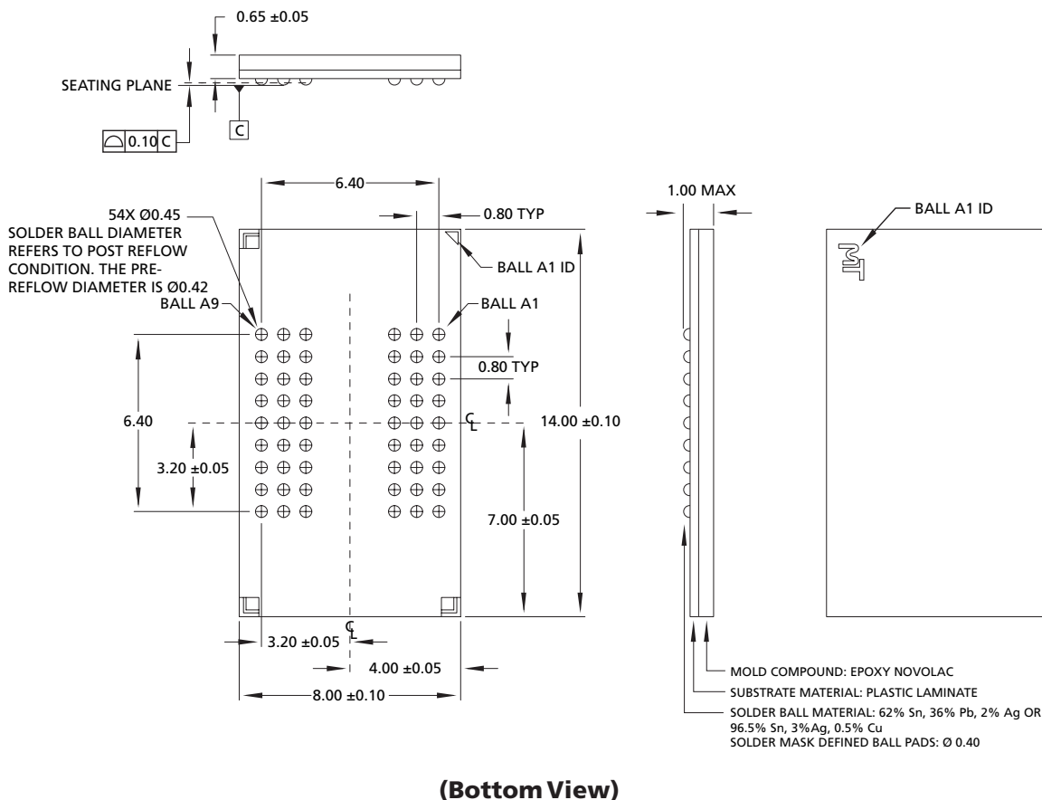
Figure 55: VFBGA "FG" Package, 54-ball, 8mm x 14mm x16
