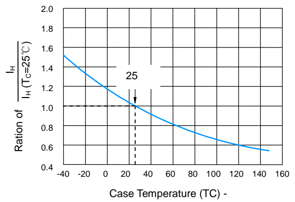
Figure4 -NormalizedDCHoldingCurrentVersusCase Temperature
