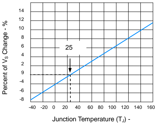
Figure3-Normalized VSChangeVersusJunction Temperature
