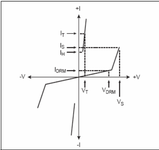
Figure1 V-I Characteristics
