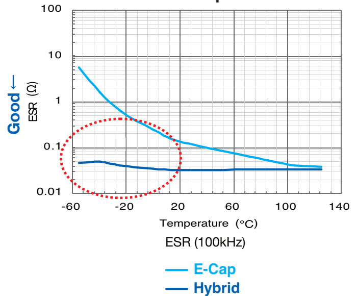
Hybrid capacitors offer stable ESR even at temperatures as low as -55°C.
