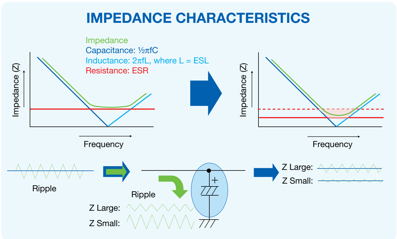
Figure 5 ESR lowers impedance near the resonance point, reducing AC ripple.
