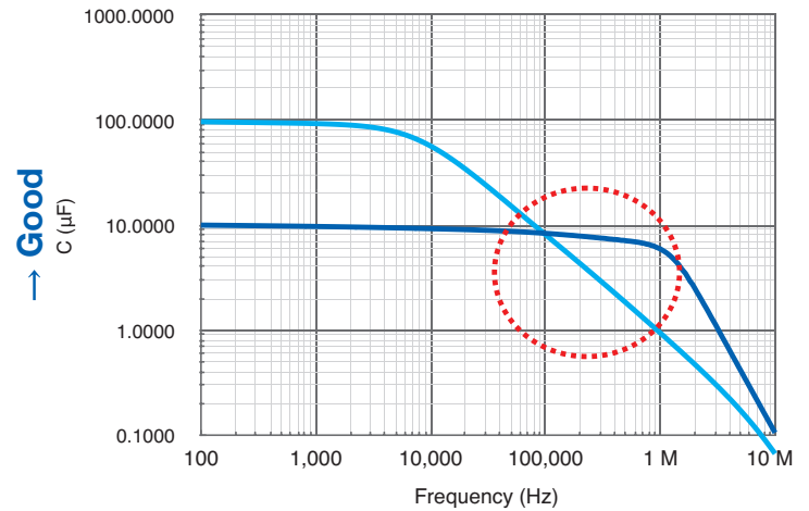
Hybrid capacitors offer stable capacitance at high frequencies.
