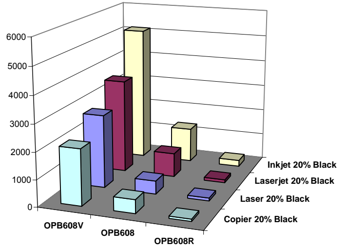
Reflective Response
