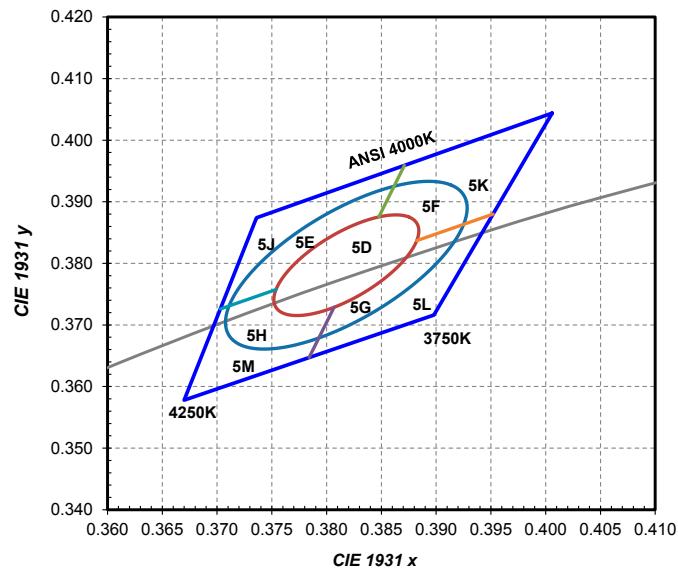
Figure 6e: 1/9 th color bin structure for LUXEON 3030 2D 4000K, hot-color targeted at 85°C.
