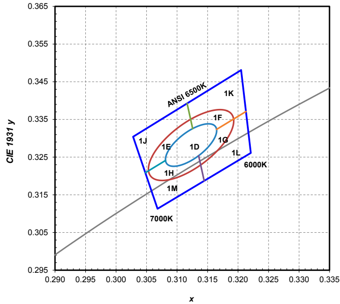
Figure 6h: 1/9 th color bin structure for LUXEON 3030 2D 6500K, hot-color targeted at 85°C.
