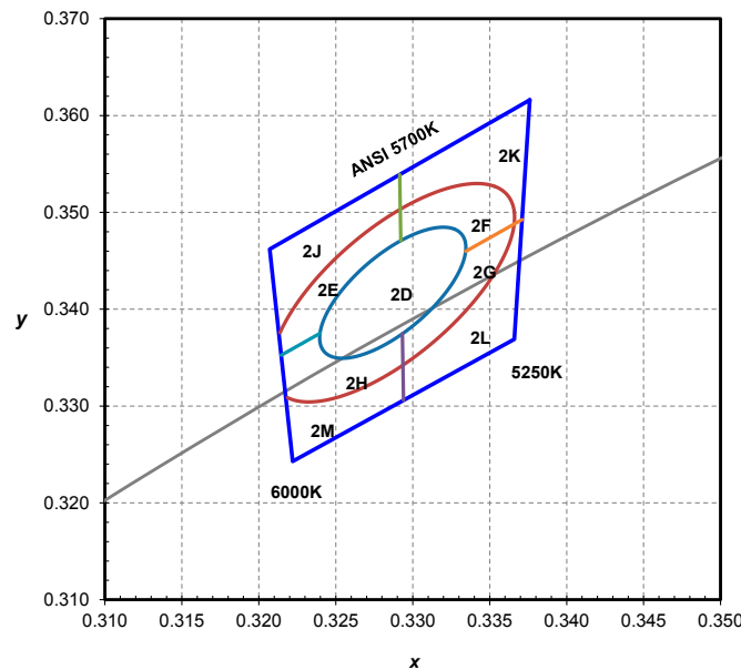
Figure 6g: 1/9 th color bin structure for LUXEON 3030 2D 5700K, hot-color targeted at 85°C.
