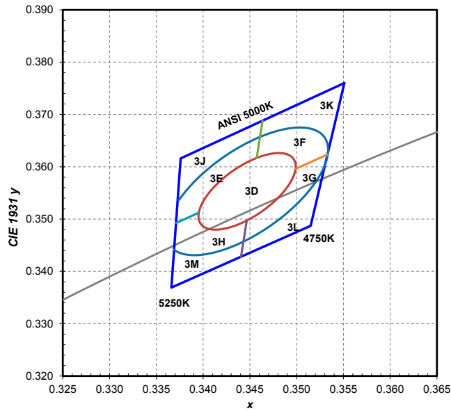
Figure 6f: 1/9 th color bin structure for LUXEON 3030 2D 5000K, hot-color targeted at 85°C.
