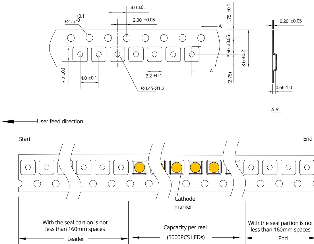
Figure 10: Tape dimensions for LUXEON 3030 2D.
