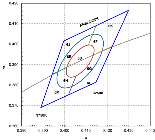
Figure 6d: 1/9 th color bin structure for LUXEON 3030 2D 3500K, hot-color targeted at 85°C.
