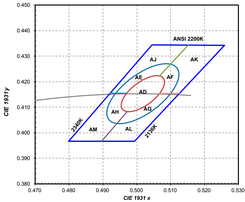
Figure 6a. 1/9 th color bin structure for LUXEON 3030 2D 2200K, hot-color targeted at 85°C.
