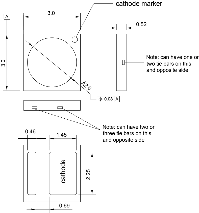
Figure 7: Mechanical dimensions for LUXEON 3030 2D.
