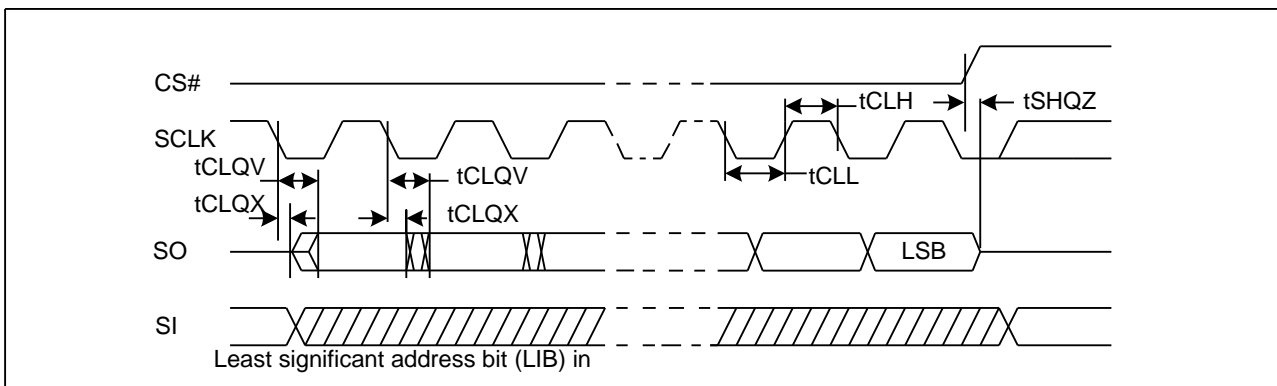
Figure36. Output Timing
