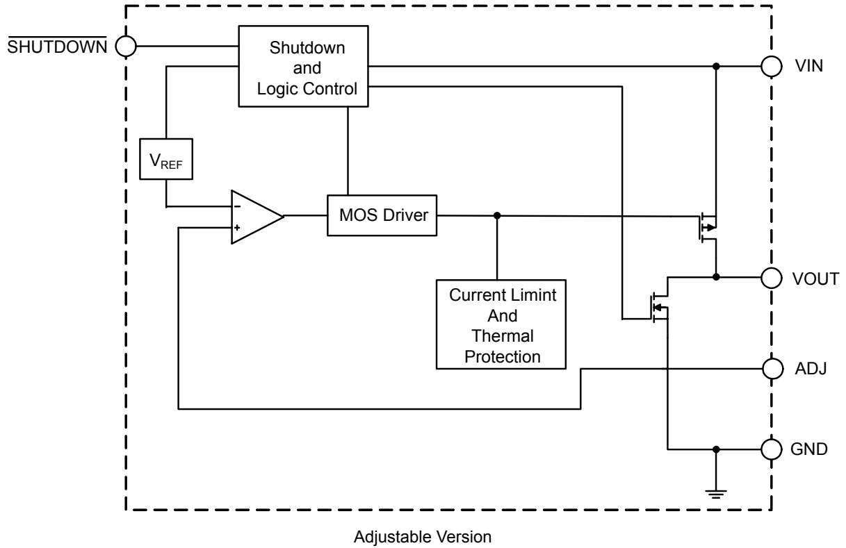
Figure 3. Functional Block Diagram of AP2128
