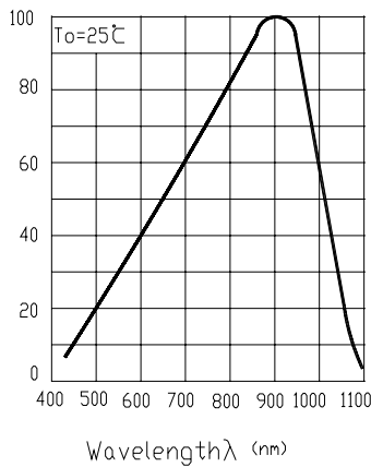
Fig.3 Spectral Sensitivity
