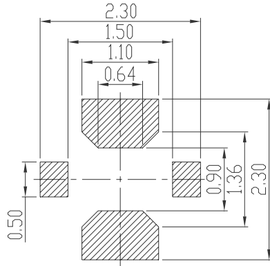
Recommend PCB Layout General Tolerance: ±0.05
