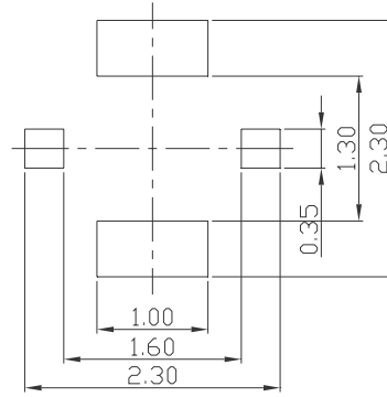
RECOMMENDED METAL MASK THICKNESS 0.12MM
