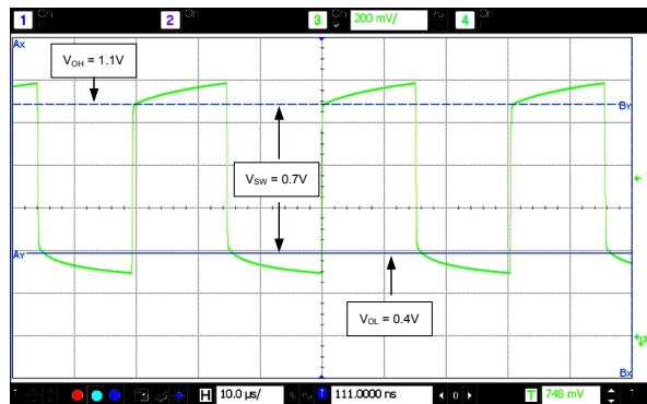
Figure 2. ANY1552AI-JE-D14-32.768 Output Waveform (10 pF Load)
