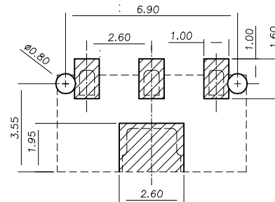
RECOMMENDED PCB LAYOUT TOP VIEW (XX±0.05)
