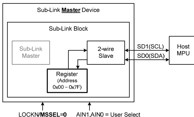
Figure 6. Host to Sub-Link Master Register access configuration
