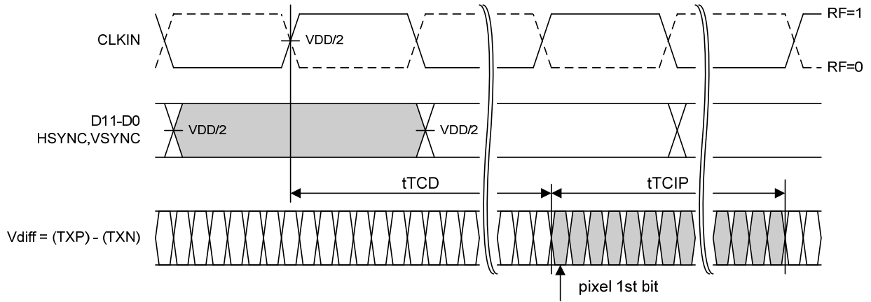
Figure 21. THCV231 Latency
