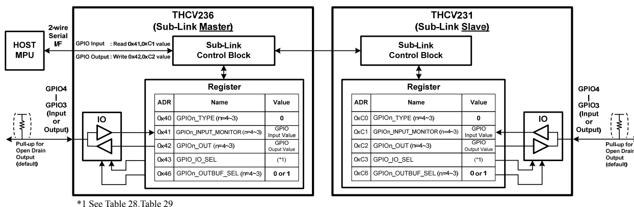
Figure 12. Programmable GPIO
