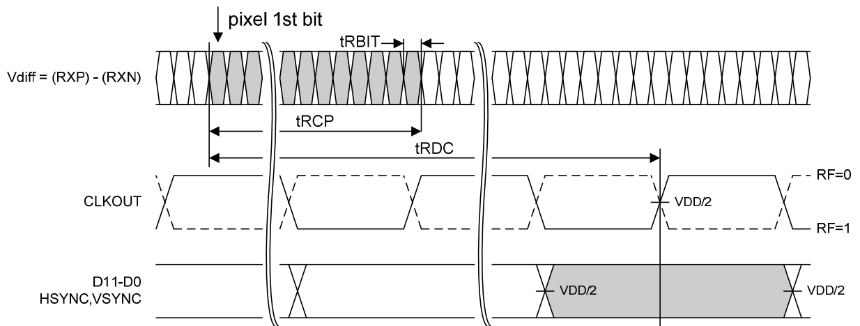
Figure 22. THCV236 Latency
