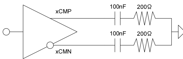
Figure 19. Bi-directional CML VBOD/VBOC Test Circuit
