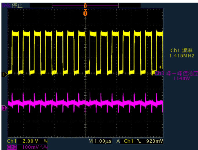
Boost waveform: Vbat=3V, Iout=1A; CH1/CH3= LX/Vp-p
