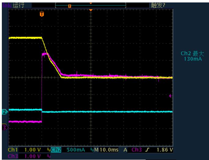
BOOST OFF waveform: CH1/CH2/CH3= Vout/Ibat/Boost
