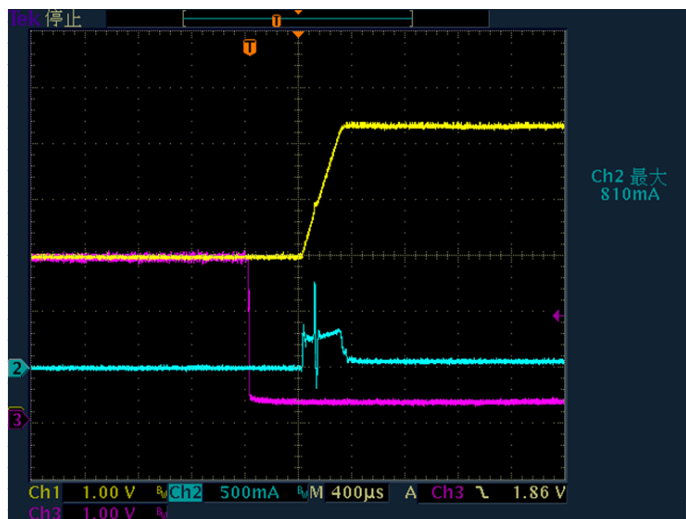
BOOST ON waveform: CH1/CH2/CH3= Vout/Ibat/Boost
