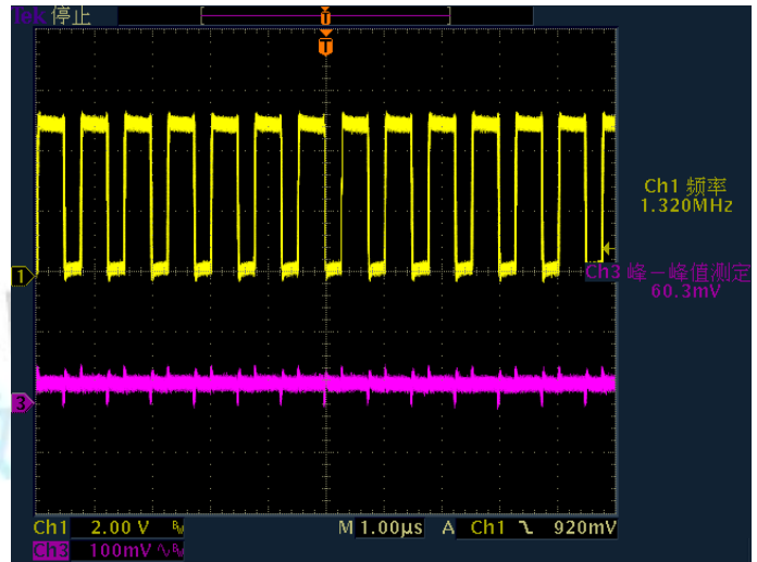
Boost waveform: Vbat=3V, Iout=200mA; CH1/CH3= LX/Vp-p
