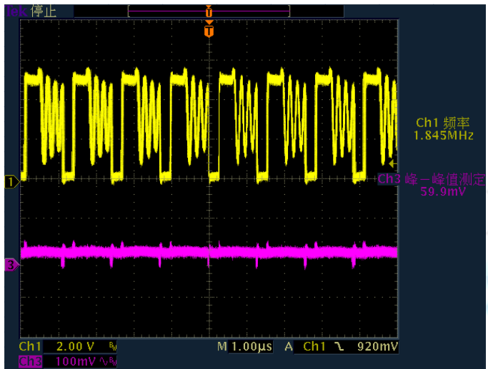
Boost waveform: Vbat=3V, Iout=100mA; CH1/CH3= LX/Vp-p
