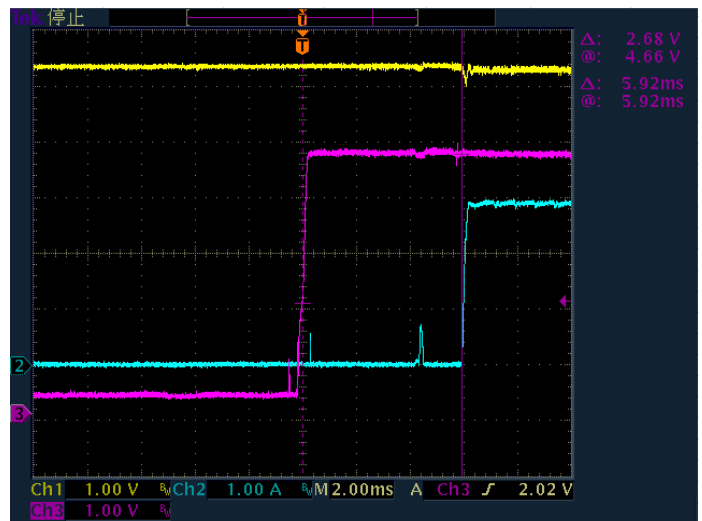
OTG: L→H; CH1/CH2/CH3= VBUS/Ibat/OTG
