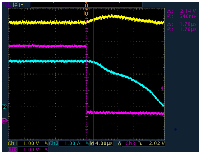
OTG: H→L; CH1/CH2/CH3= VBUS/Ibat/OTG
