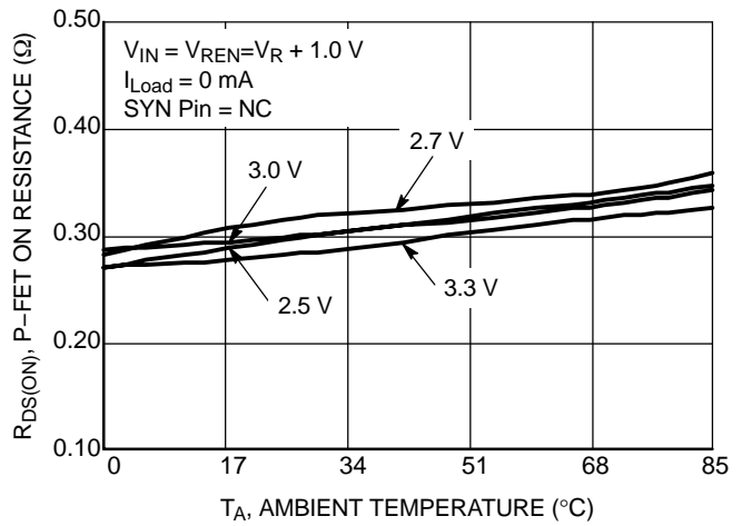
Figure 10. P-FET ON Resistance vs. Ambient Temperature
