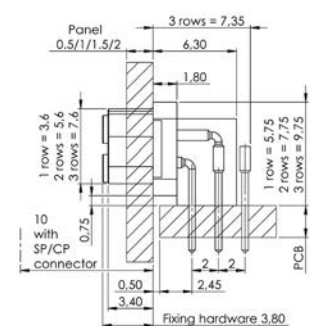
90° female
