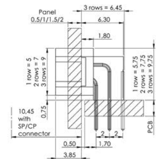
90° male
