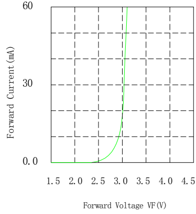
Forward current vs. Forward Voltage (Ta=25° C)
