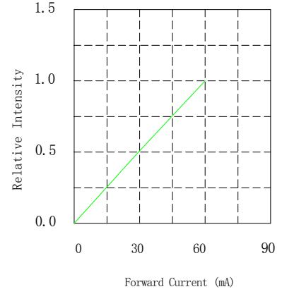
Relative Intensity vs. Forward Current (Ta=25° C)
