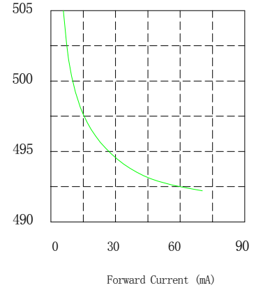
Forward Current vs. Chromaticity (Ta=25° C)
