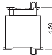
MATING HEIGHT:4.5mm
