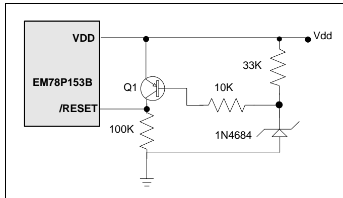
Figure 5-11a Residue Voltage Protection Circuit 1
