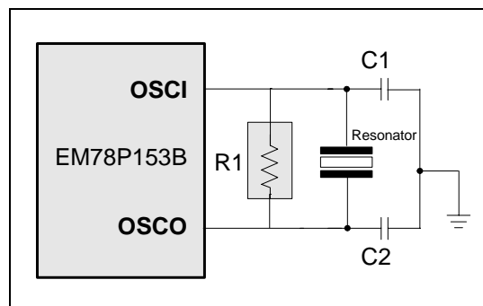
Figure 5-8b Circuit for Crystal/Resonator
