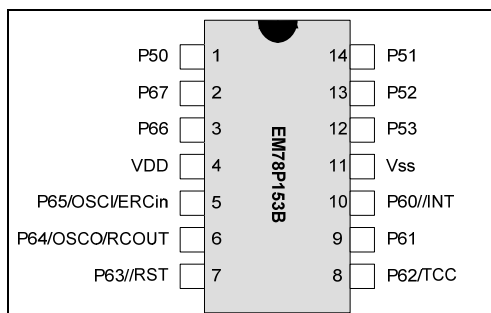
Figure 3-1a EM78P153BD14J, EM78P153BSO14J
