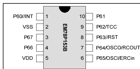
Figure 3-1b EM78P153BSS10J
