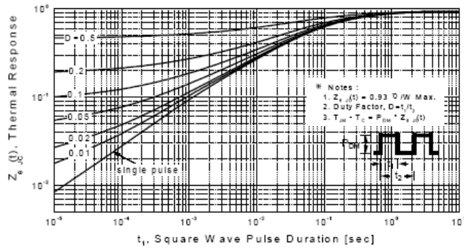
Figure 11-1. Transient Thermal Response Curve for SLP840C
