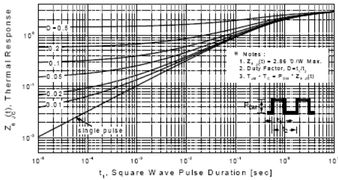
Figure 11-2. Transient Thermal Response Curve for SLF840C
