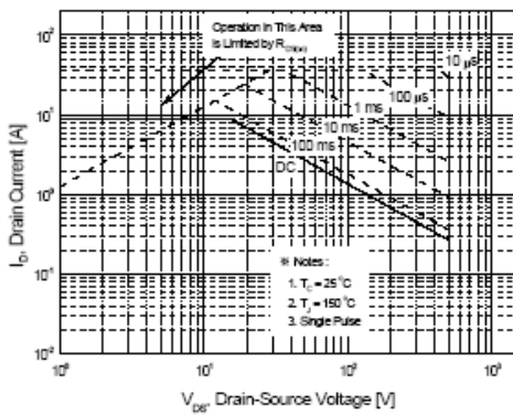
Figure 9-1. Maximum Safe Operating Area for SLP840C
