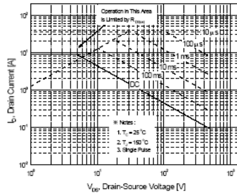
Figure 9-2. Maximum Safe Operating Area for SLF840C
