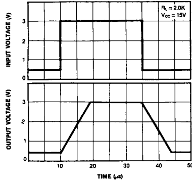
Figure 7. Slew Rate
