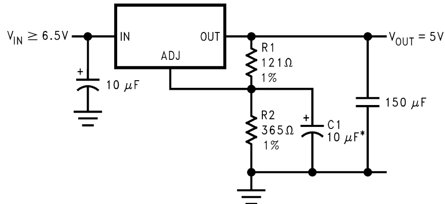
Figure 23. Ripple Rejection Enhancement
