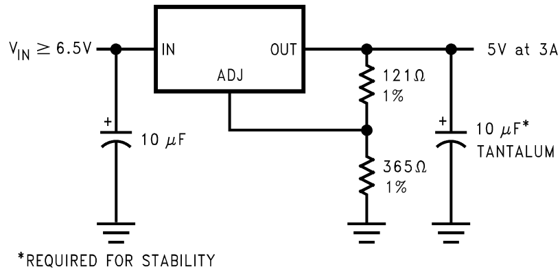
Figure 16. Adjustable @ 5V
