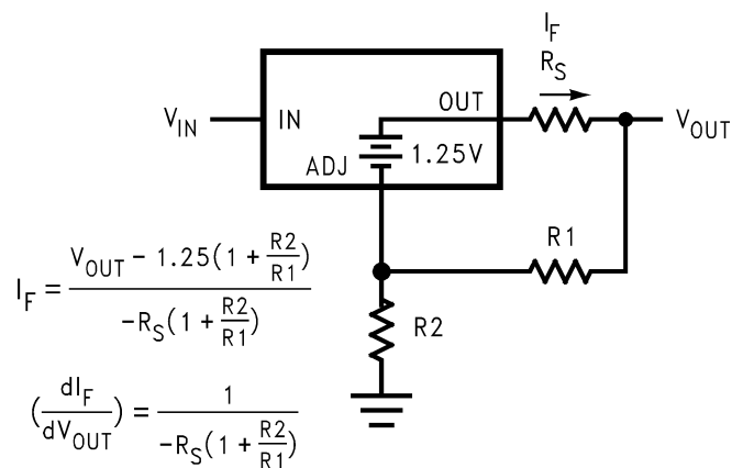
Figure 18. Battery Charger
