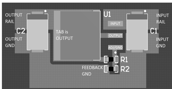
Figure 27. Layout Example
