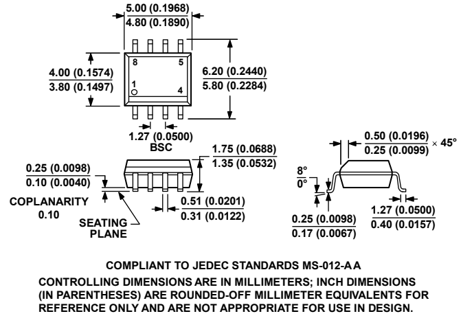
COMPLIANT TO JEDEC STANDARDS MS-012-AA CONTROLLING DIMENSIONS ARE IN MILLIMETERS; INCH DIMENSIONS (IN PARENTHESES) ARE ROUNDED-OFF MILLIMETER EQUIVALENTS FOR REFERENCE ONLY AND ARE NOT APPROPRIATE FOR USE IN DESIGN. Figure 72. 8-Lead Standard Small Outline Package [SOIC_N] Narrow Body (R-8) Dimensions shown in millimeters and (inches)
