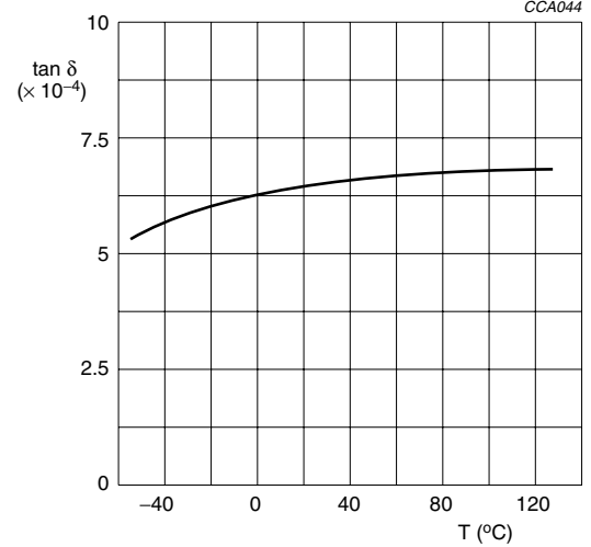
Fig. 4 Typical tan δ as a function of temperature
