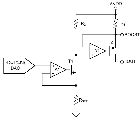
Figure 84. Current Output
