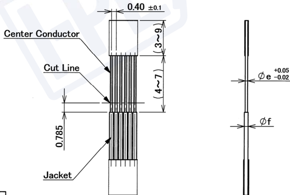
RECOMMENDED DISCRETE CABLE AWG #**
