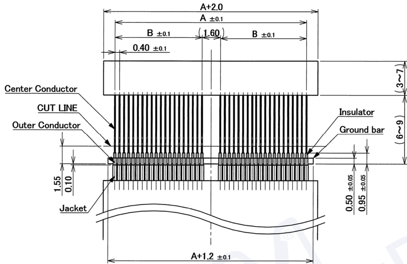
RECOMMENDED MICRO-COAX CABLE AWG #**
