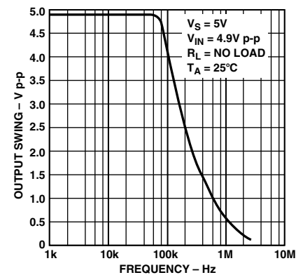
TPC 18. Closed-Loop Output Voltage Swing vs. Frequency
