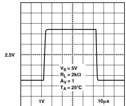
TPC 24. Large Signal Transient Response
