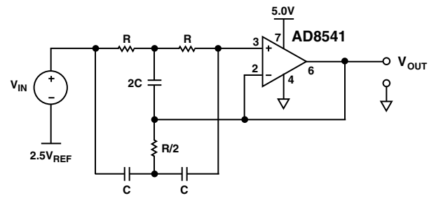
Figure 2. 60 Hz Twin-T Notch Filter, Q = ∞ (Ideal)
