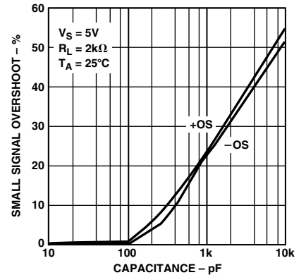
TPC 21. Small Signal Overshoot vs. Load Capacitance
