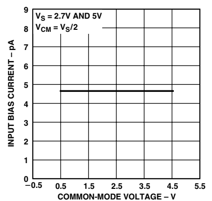
TPC 3. Input Bias Current vs. Common-Mode Voltage
