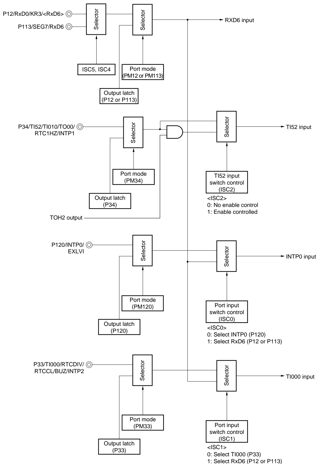
Figure 14-3. Port Configuration for LIN Reception Operation
