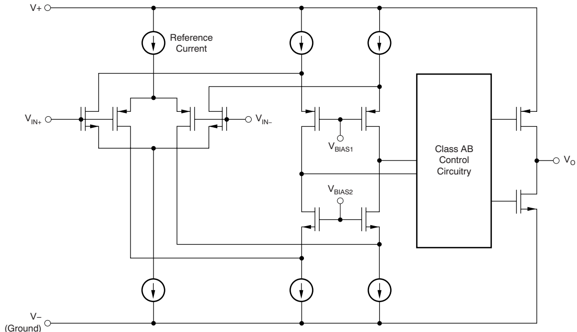
Figure 34. Simplified Schematic
