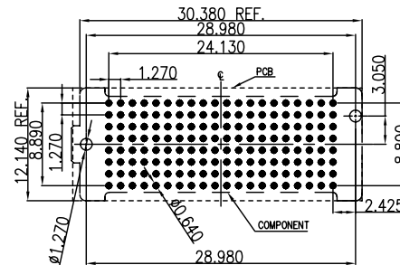
RECOMMENDED PCB LAYOUT (TOP VIEW) (ALL TOLERANCE ARE ±0.05)
