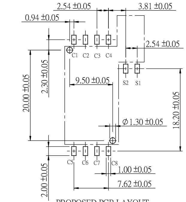
PROPOSED PCB LAYOUT
