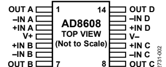
Figure 6. 14-Lead TSSOP (RU Suffix)
