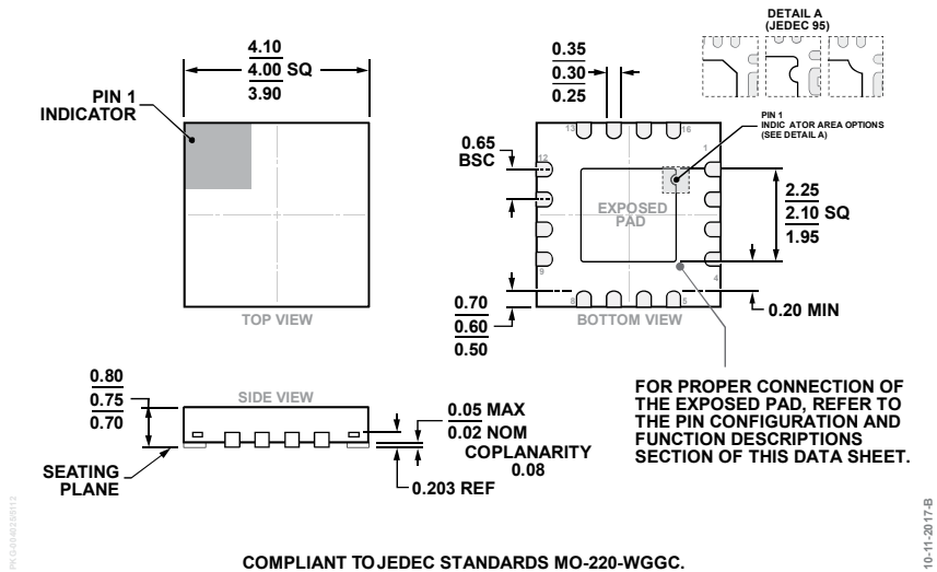
Figure 57. 16-Lead Lead Frame Chip Scale Package [LFCSP] 4 mm × 4 mm Body and 0.75mm Package Height (CP-16-23) Dimensions shown in millimeters
