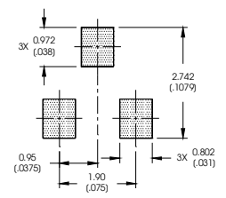
RECOMMENDED FOOTPRINT
