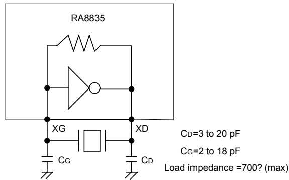
Figure 7-4: Crystal Oscillator
