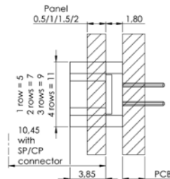
Straight male
