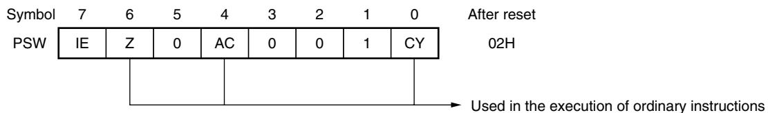
Figure 13-6. Program Status Word (PSW) Configuration
