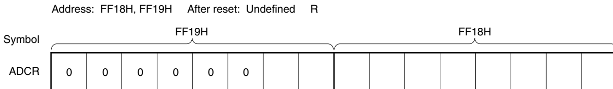
Figure 10-6. Format of 10-bit A/D Conversion Result Register (ADCR)
