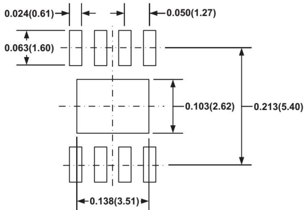
Land Pattern
