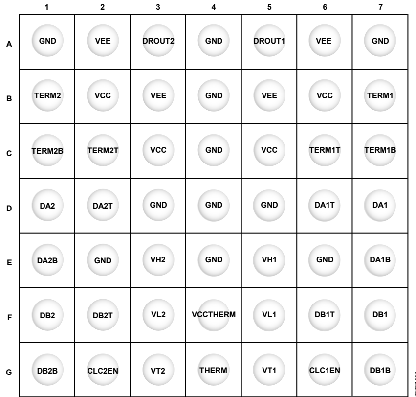
Figure 2. Pin Configuration
