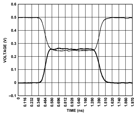
Figure 14. V_{Hx} = 1.0\text{ V} , V_{Tx} = 0.5\text{ V} , V_{Lx} = 0.0\text{ V} , Transitions Between V_{Hx}/V_{Lx} and V_{Tx}
