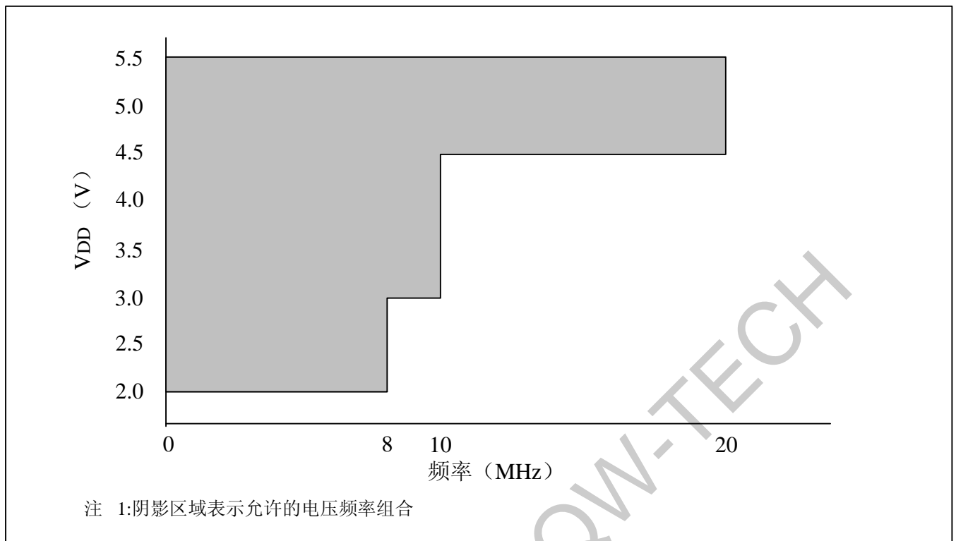
图 13-1-1: MDT10F684 电压-频率图, -40\text{ }^{\circ}\text{C} \leq \text{TA} \leq +85\text{ }^{\circ}\text{C}
