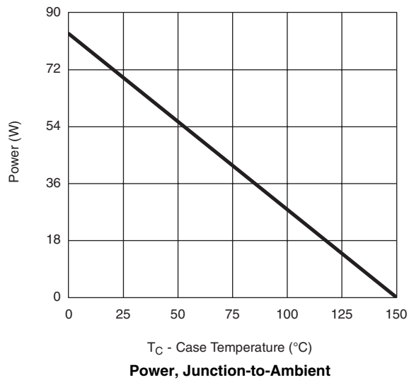
Power, Junction-to-Ambient
