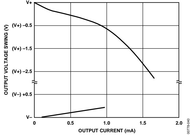
Figure 40. Output Voltage Swing vs. Output Current
