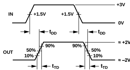
Figure 6. Driver Differential Output Delay and Transition Times
