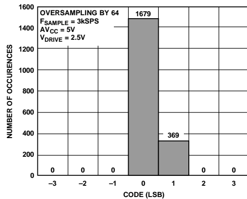
Figure 55. Histogram of Codes—OS x 64 (Two Codes)
