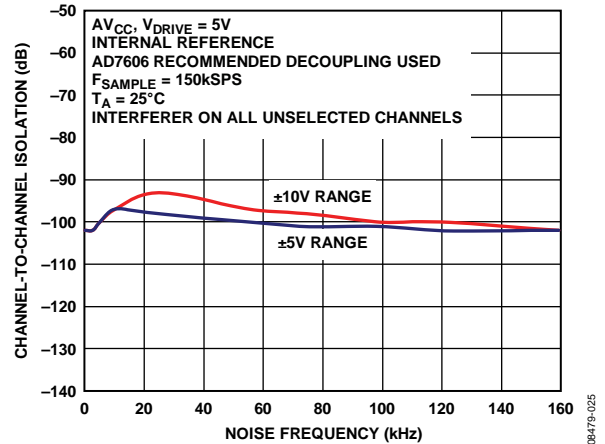
Figure 28. Channel-to-Channel Isolation
