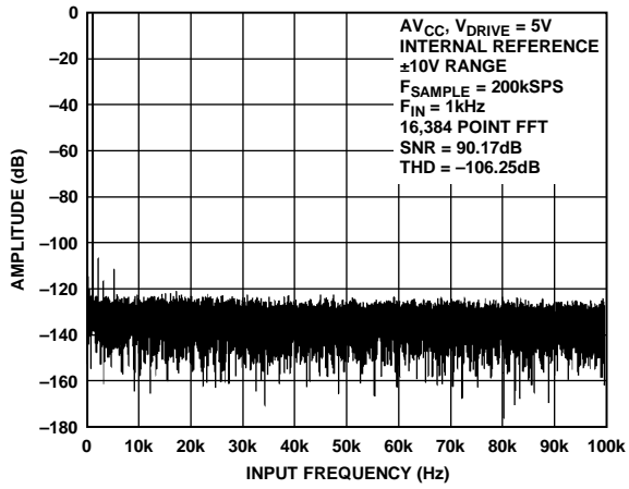
Figure 11. AD7606 FFT, \pm 10\text{ V} Range
