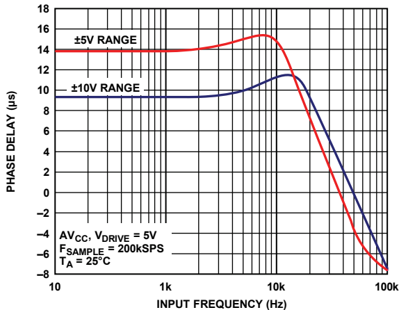
Figure 38. Analog Antialiasing Filter Phase Response
