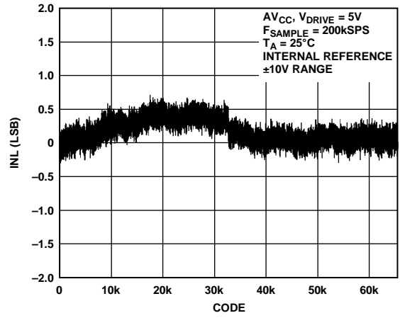
Figure 14. AD7606 Typical INL, \pm 10\text{ V} Range
