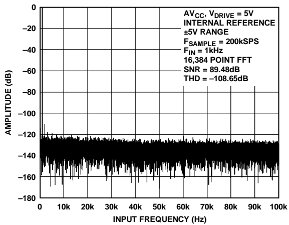
Figure 12. AD7606 FFT Plot, \pm 5\text{ V} Range
