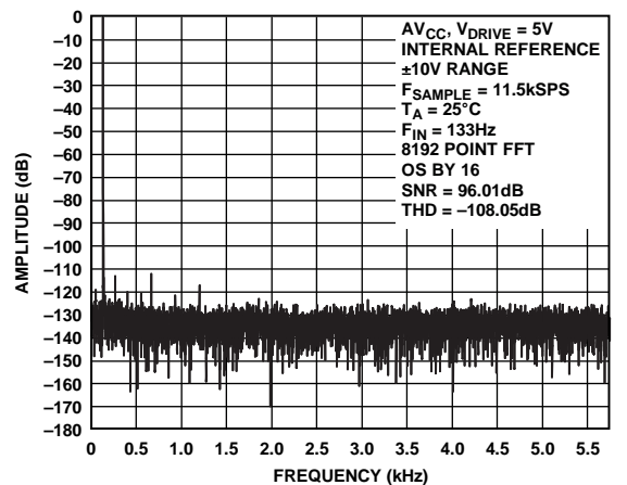
Figure 13. FFT Plot Oversampling By 16, \pm 10\text{ V} Range
