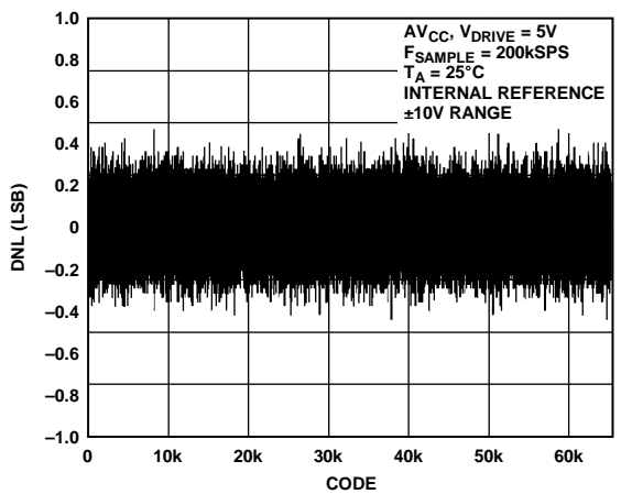
Figure 15. AD7606 Typical DNL, \pm 10\text{ V} Range
