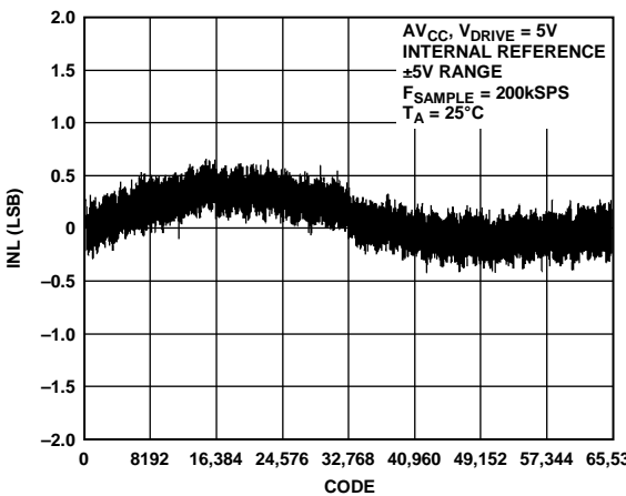
Figure 16. AD7606 Typical INL, \pm 5\text{ V} Range
