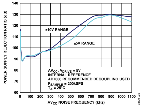
Figure 33. PSRR
